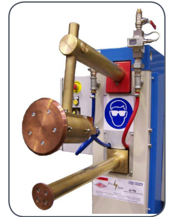
Lower Driven Circumferential Seam Welder
