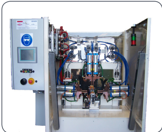
Twin Headed projection welding machine with servo controlled fixture for multi component welding
