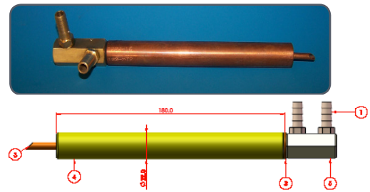
TP22-16-180-MT2 SIP Toolpost
